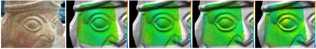
Figure 4: Eye example (area of ca 3x3 cm): results of the comparison between the range data and the image-based results (NGATE, ATE, ARC 3D, and SAT-PP respectively). The colour legends on the right of each picture show differences between + 0.15mm and - 0.15mm.
