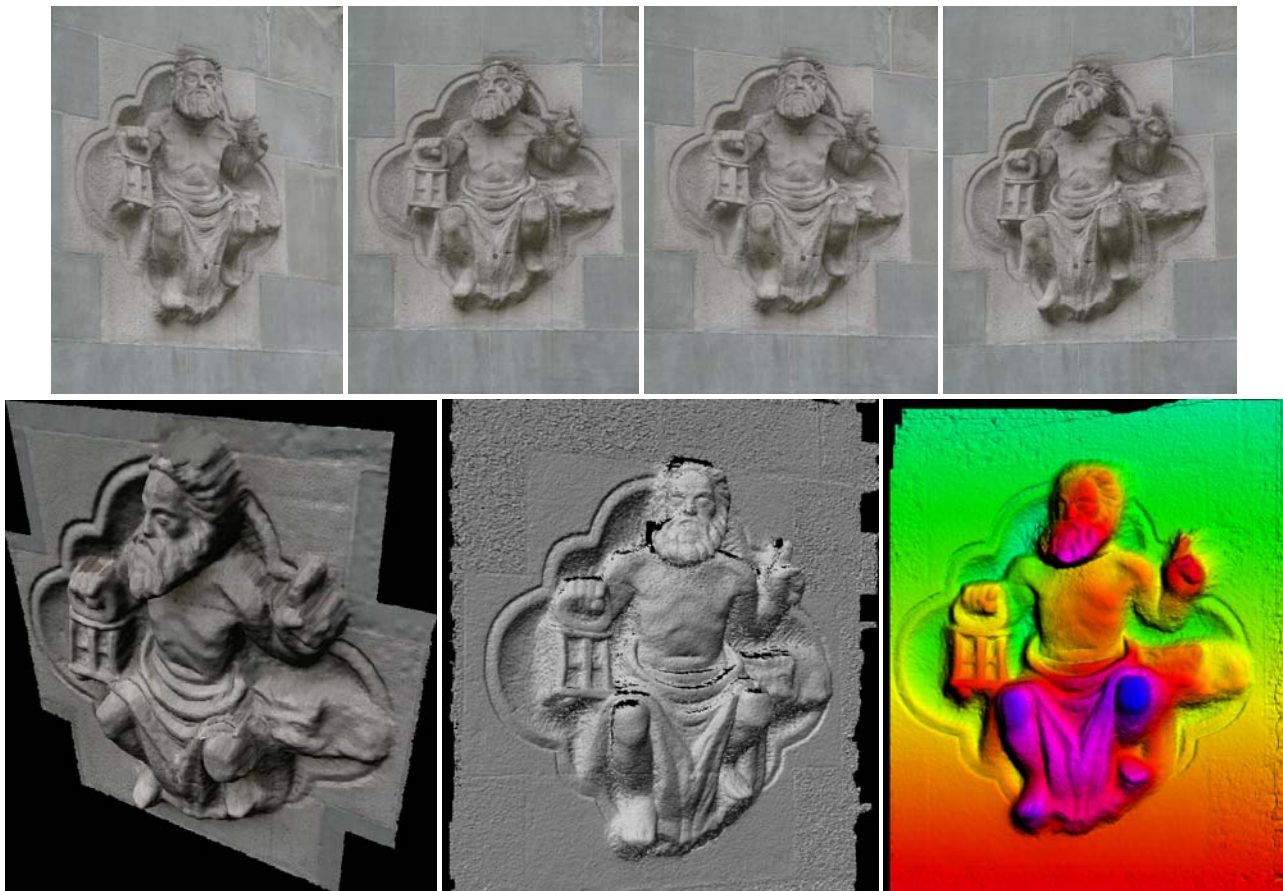
Figure 6: Bern relief (7 images) and relative surface models achieved in NGATE, ARC 3D and SAT-PP.
