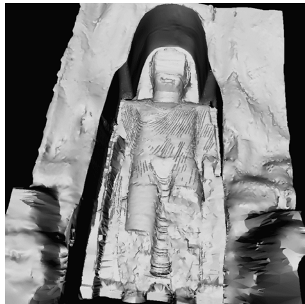
Figure 12: The shaded model of the Buddha, reconstructed with manual measurements on the three metric images.
